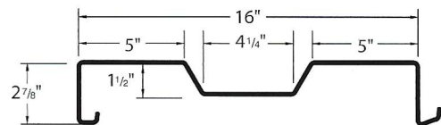
AW-16 Panel Profile
