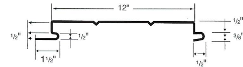
A-12 Soffit Panel
