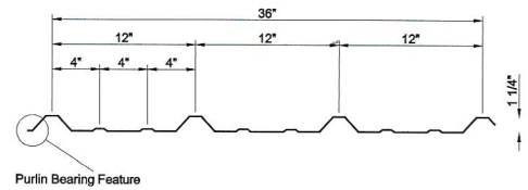
PBR Panel
