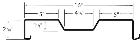
AW-16 Panel Profile
