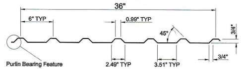
PBM Panel
