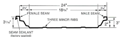
Alliance Seam 24 Standing Seam Roof System
